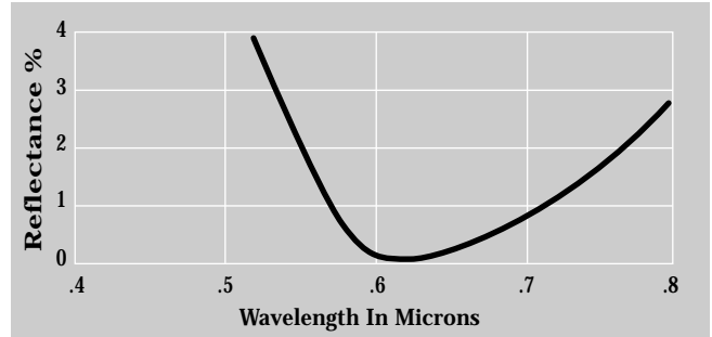
V-coat 633 nm
