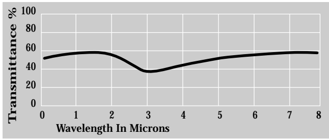
Beamsplitter Coating CaF 2 2-8 \mu\text{m}
