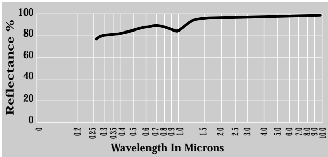
Protected Silver 0.4-10.0 \mu\text{m}
